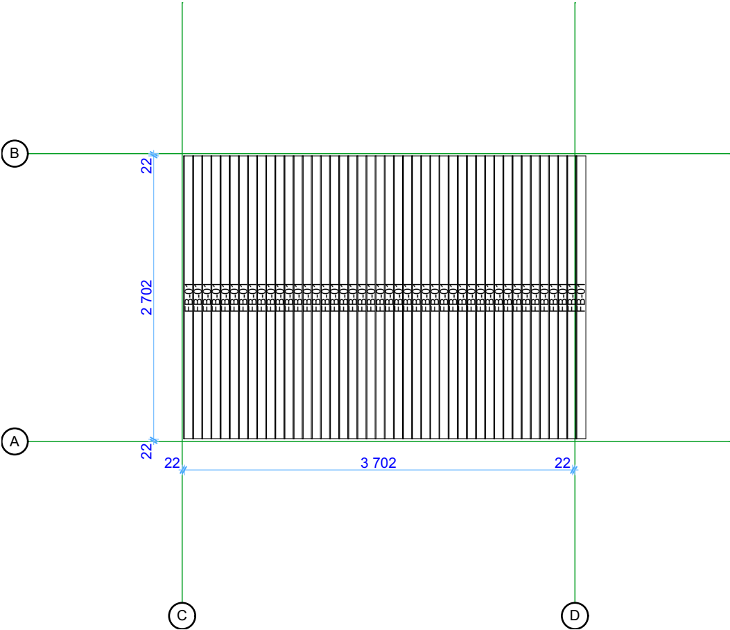
Floor board plan
