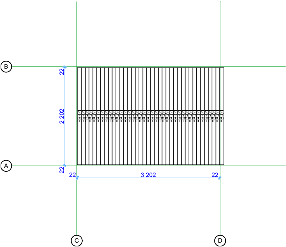
Floor board plan
