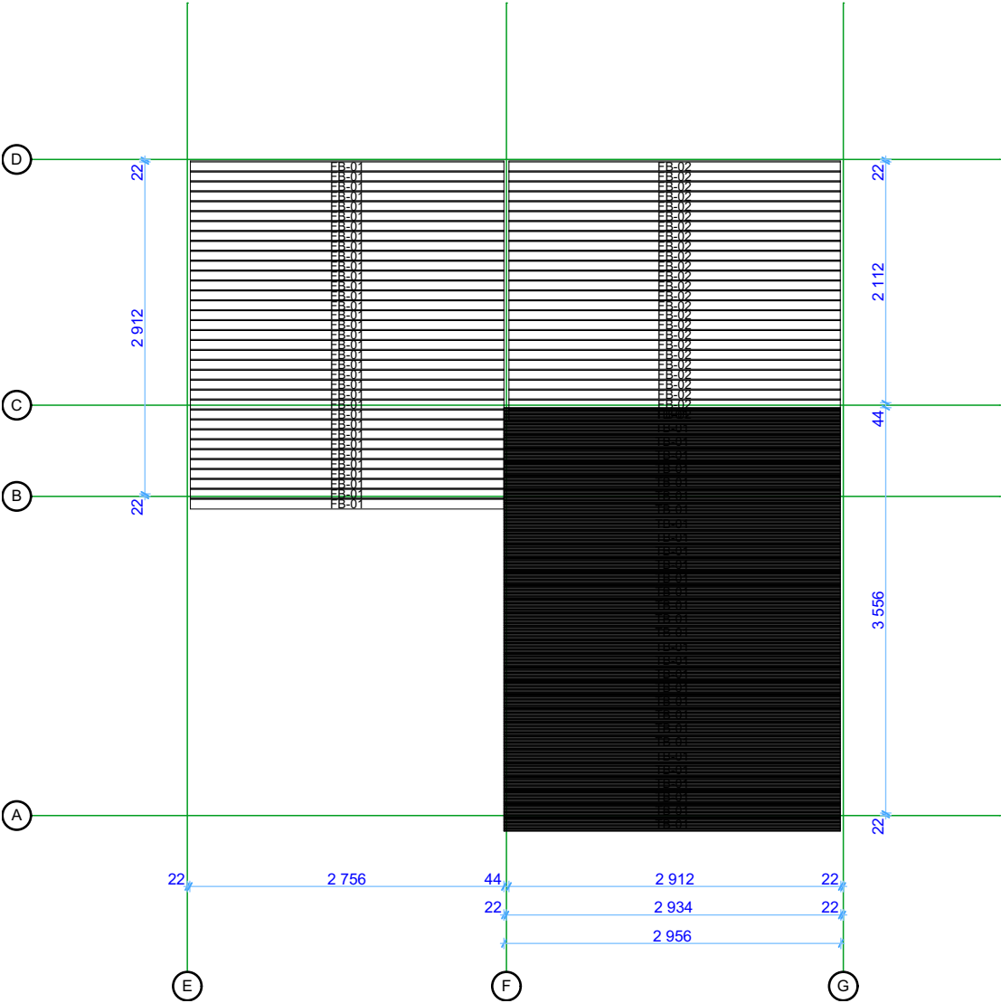
Floor board plan
