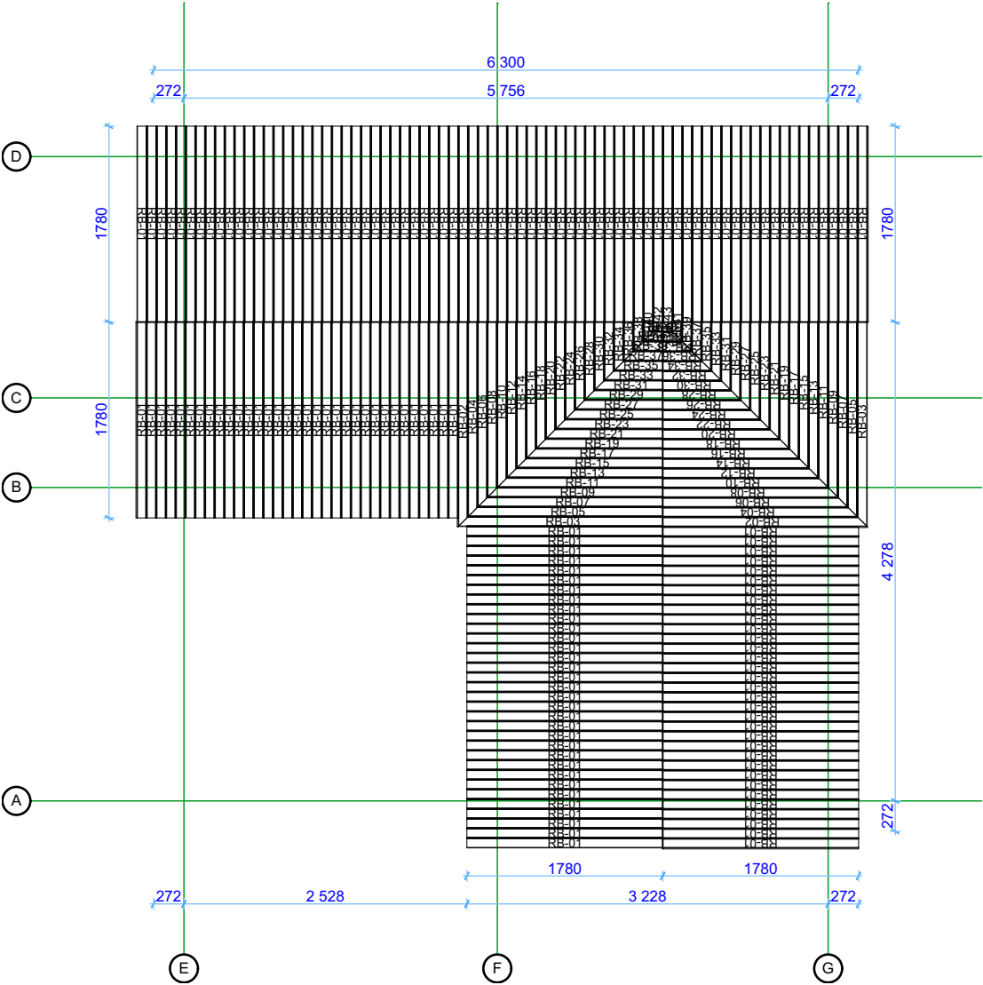
Roof board plan
