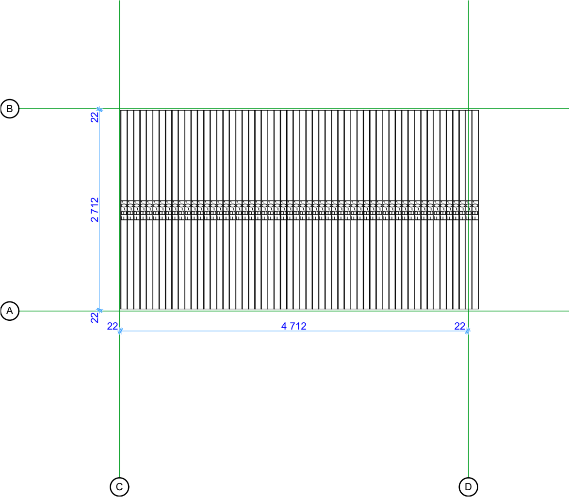
Floor board plan
