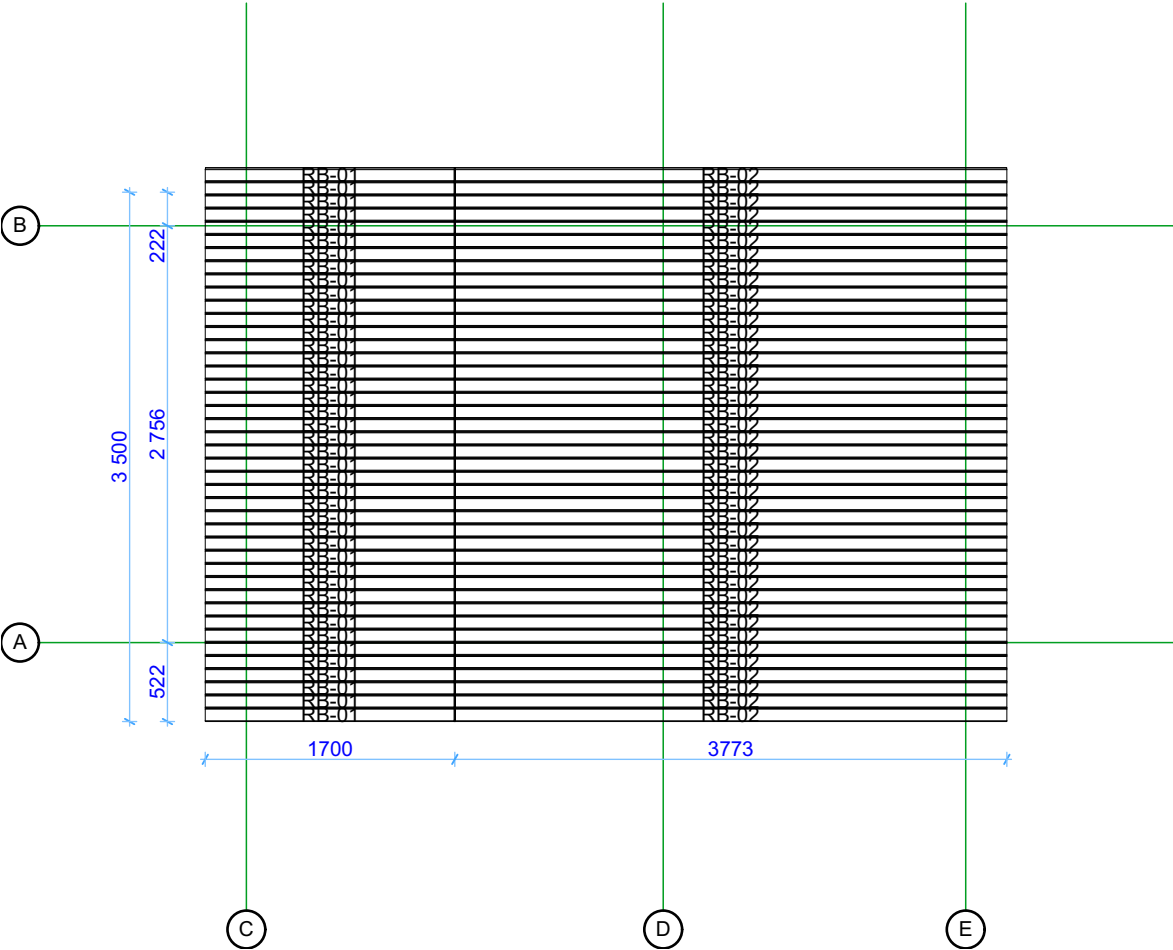
Roof board plan
