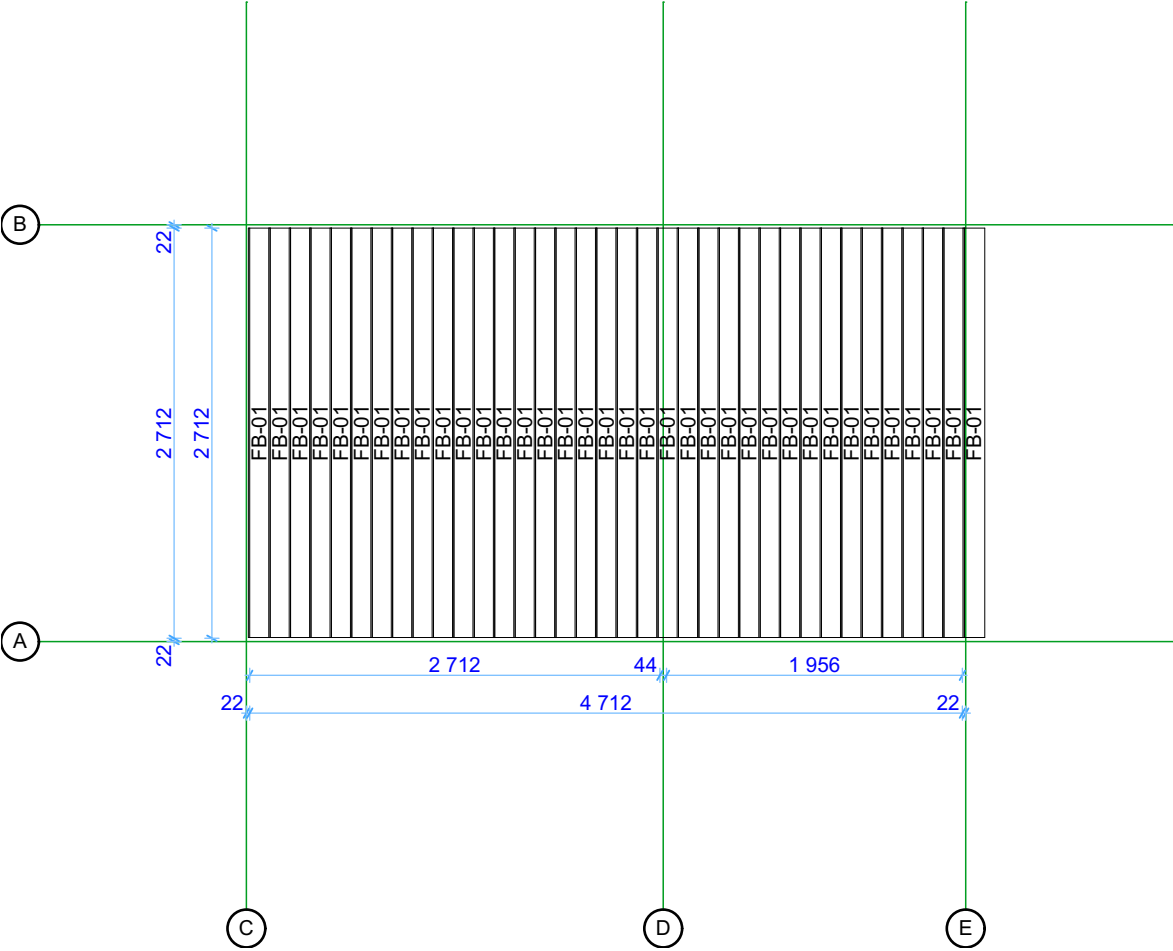
Floor board plan
