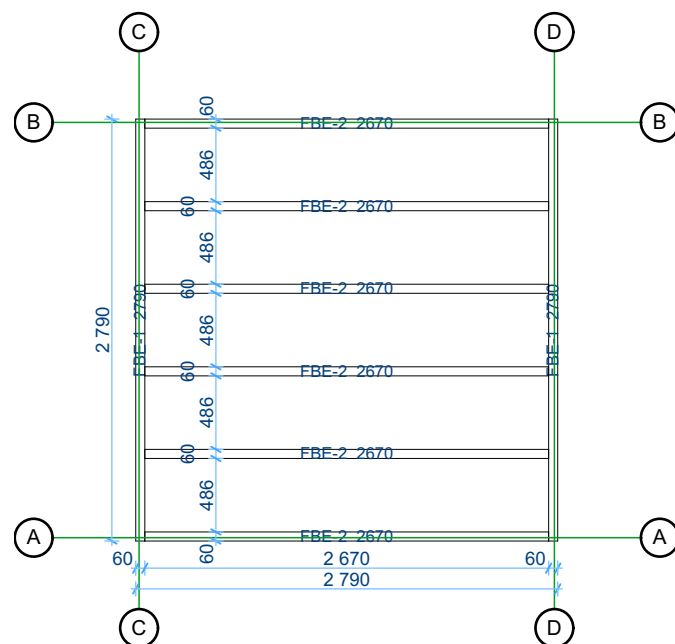
Floor bearers plan
