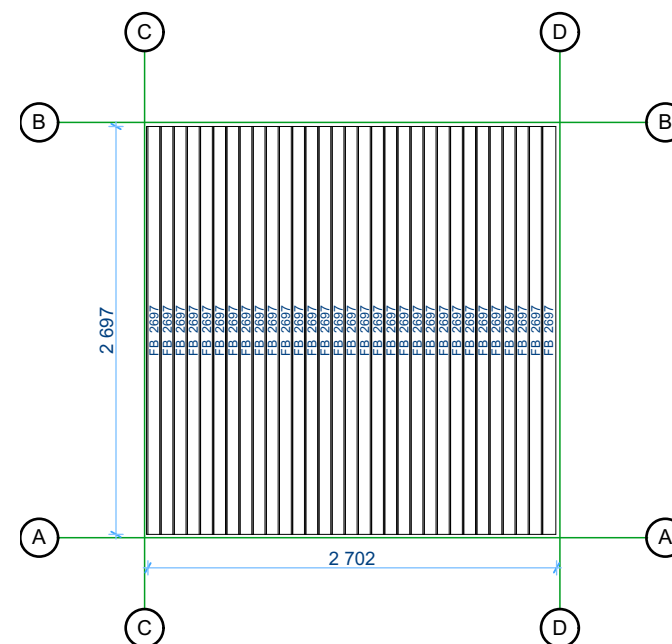
Floor boards plan
