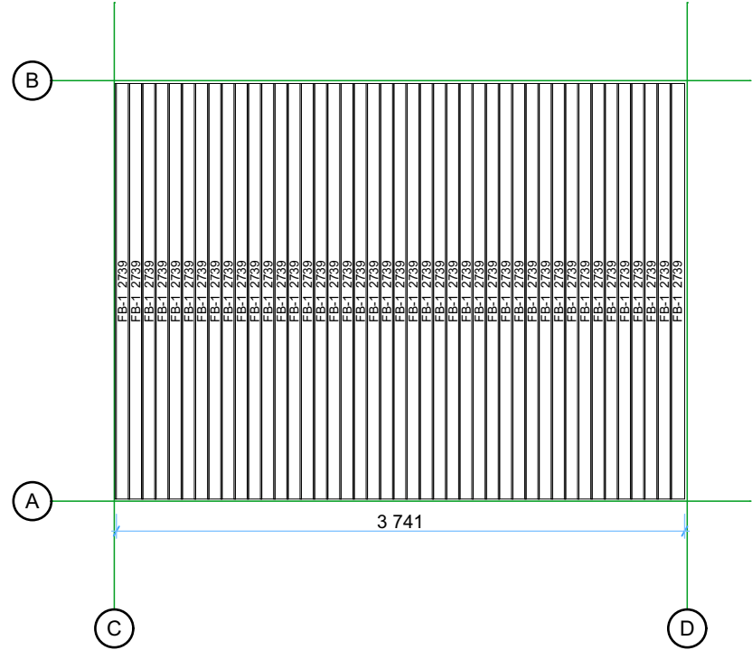
Floor boards 1:45
