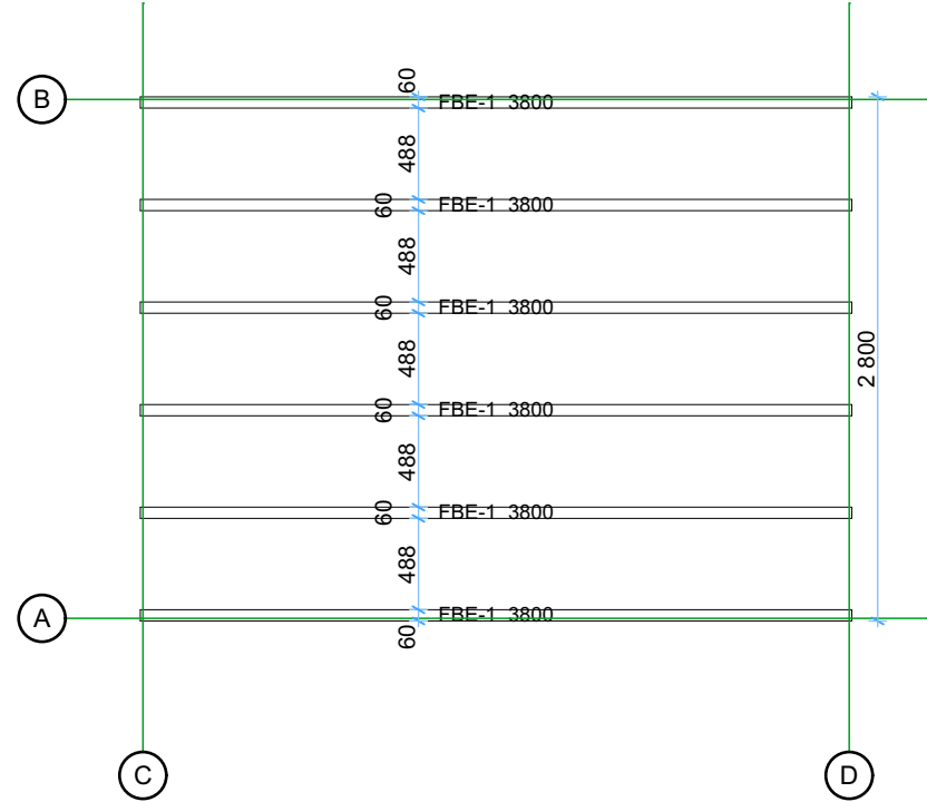
Floor bearers 1:45
