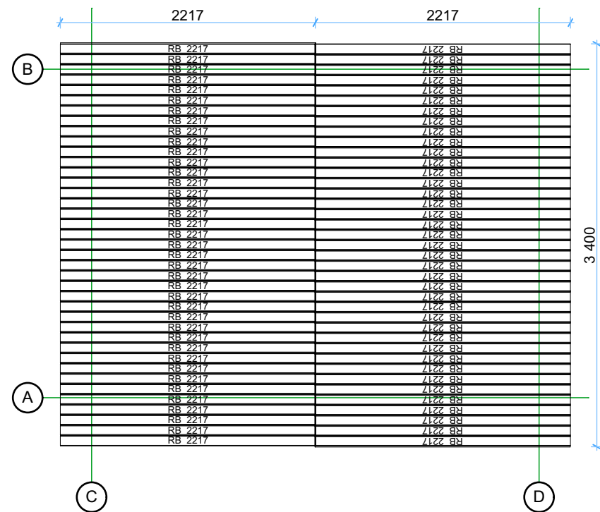
Roof boards
