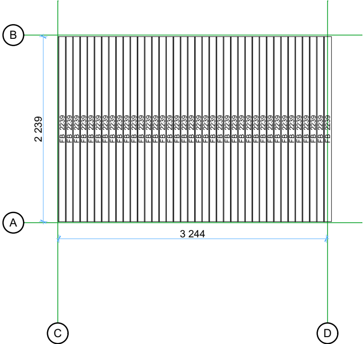
Floor boards plan
