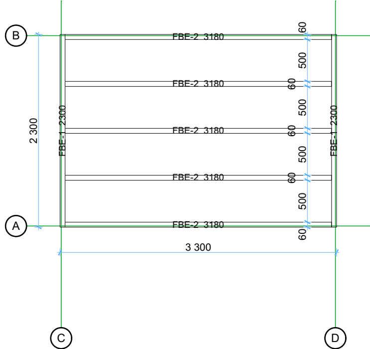
Floor bearers plan
