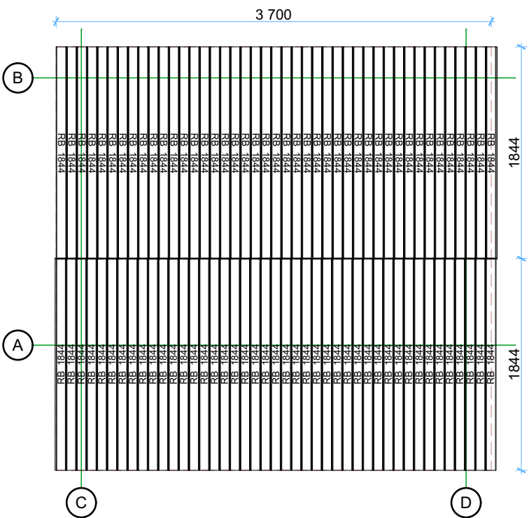
Roof boards plan
