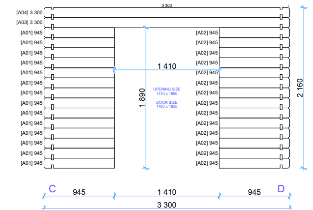
Wall C 1:50
