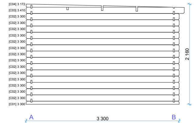
Wall C 1:50
