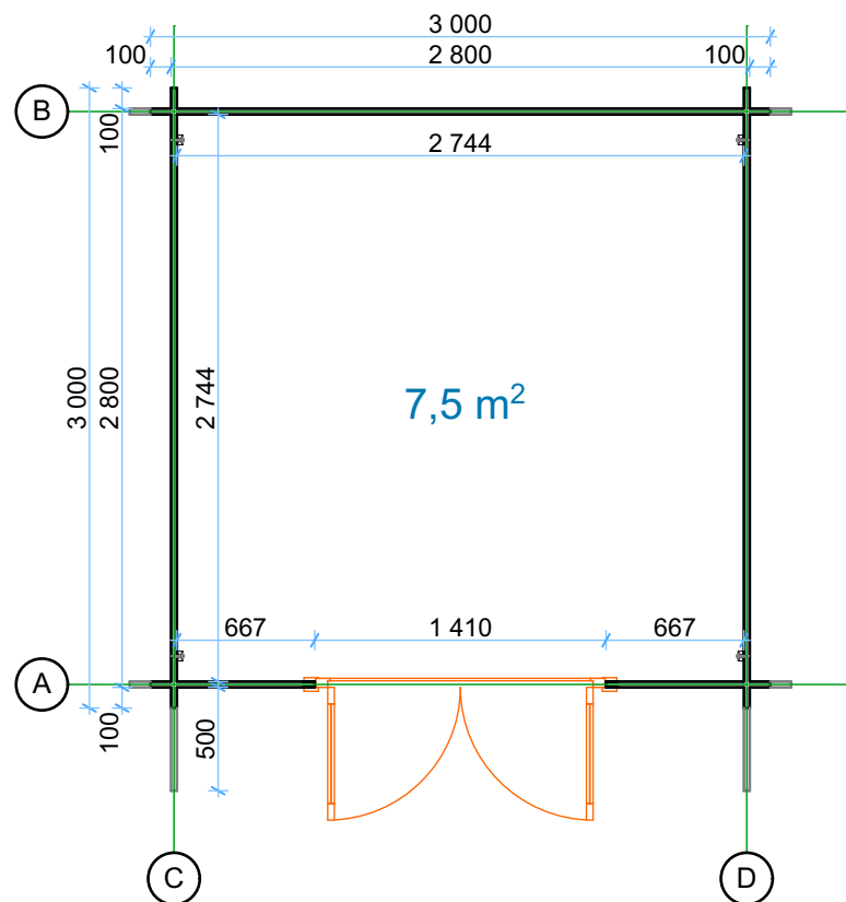
Ground floor plan 1:40
