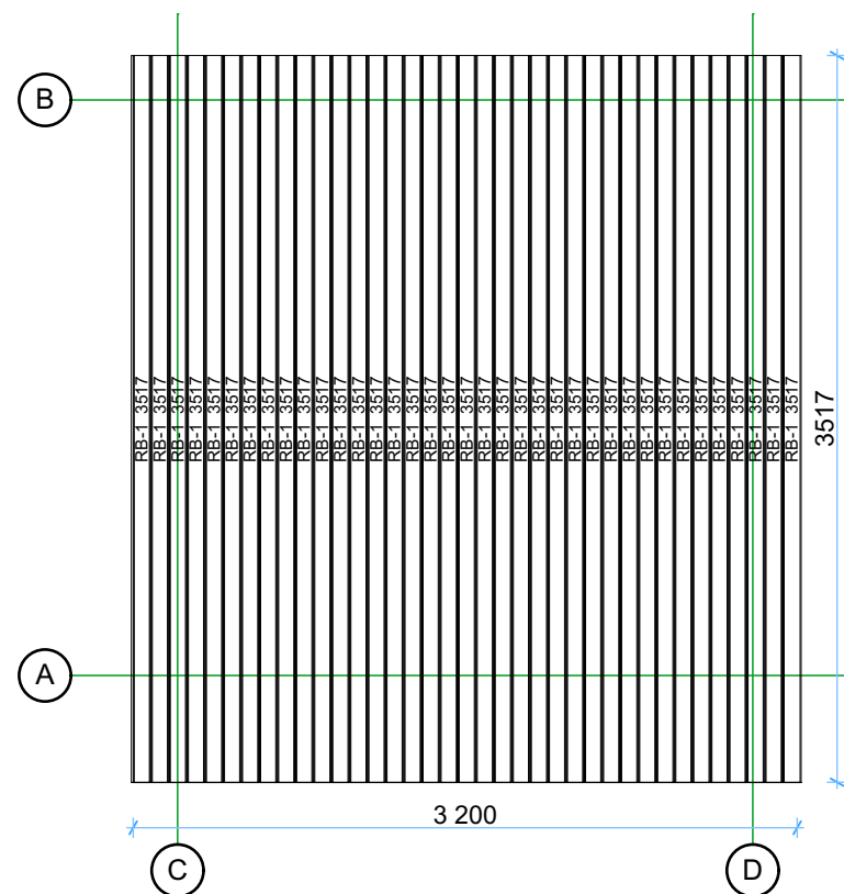
Roof boards 1:40
