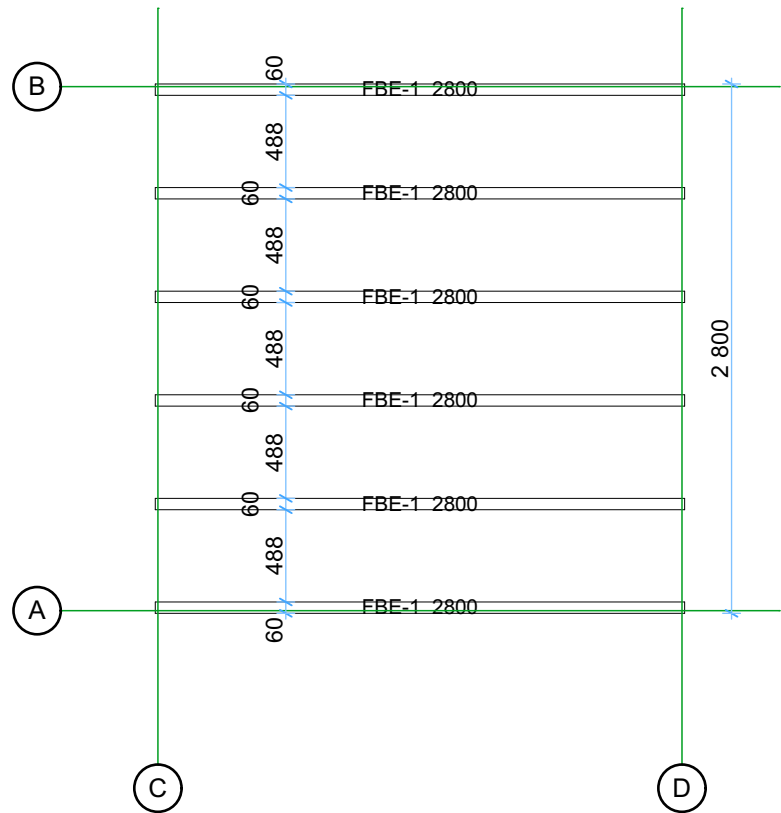
Floor bearers 1:40
