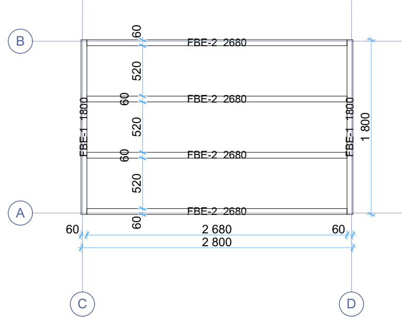
Floor bearers
