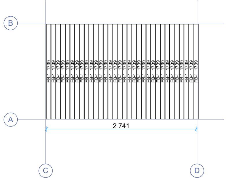
Floor boards
