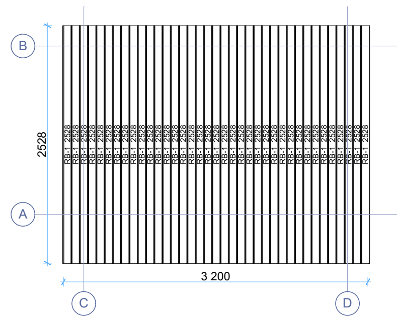
Roof boards
