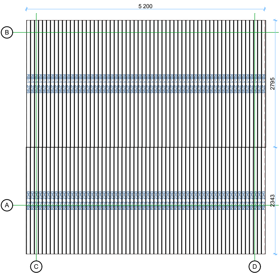
Roof boards plan
