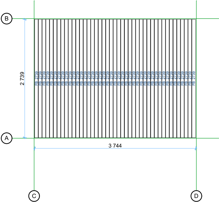
Floor boards plan
