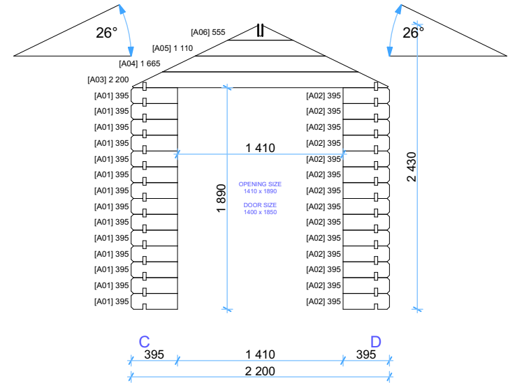
Wall B
