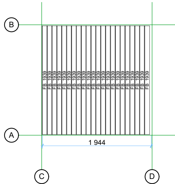
Floor boards 1:40
