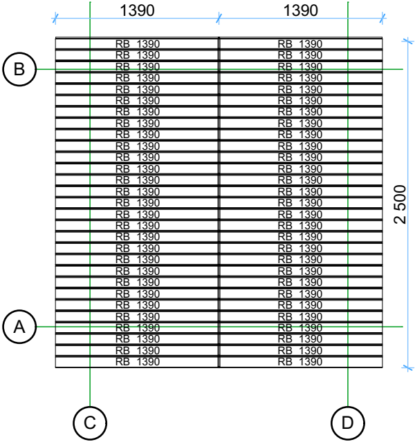
Roof boards
