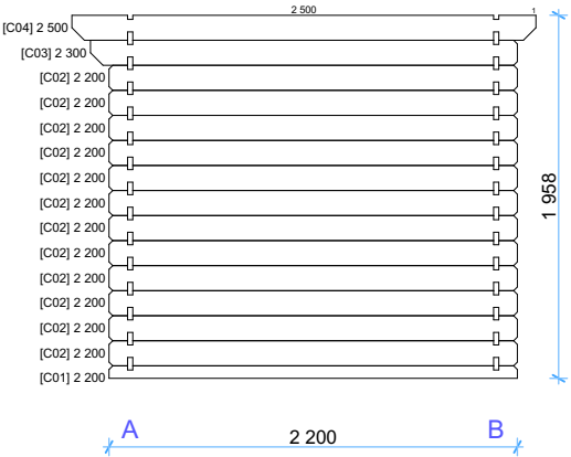
Wall D
