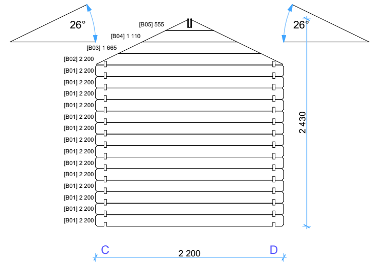
Wall B
