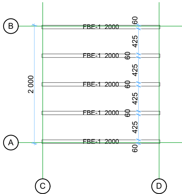
Floor bearers 1:40
