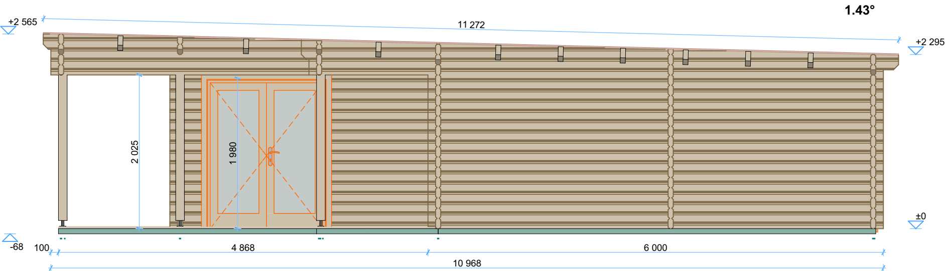
Left Elevation
