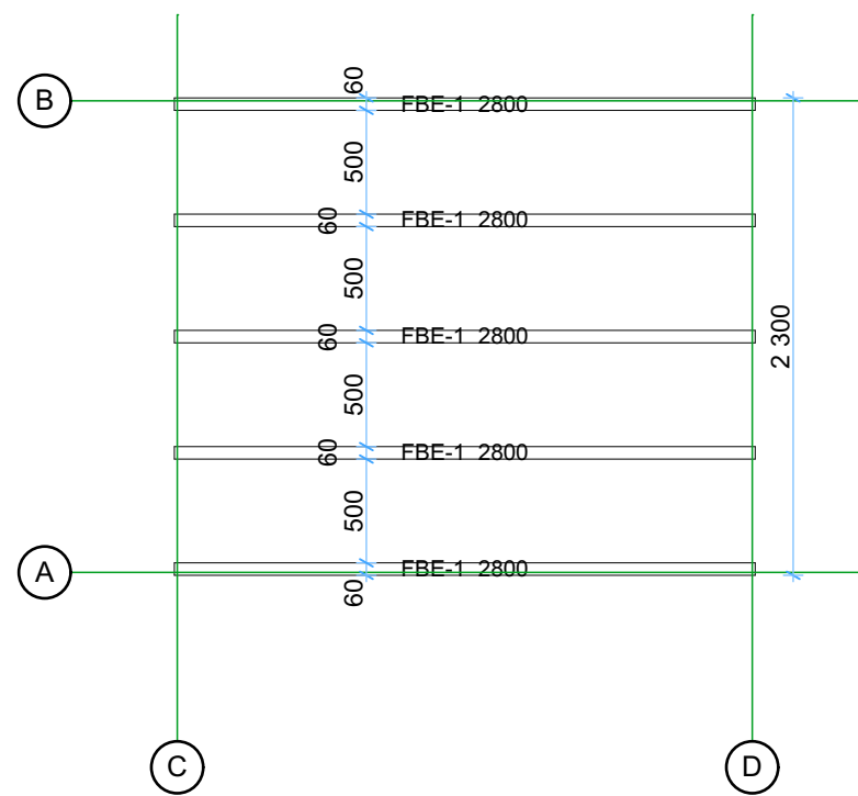
Floor bearers
