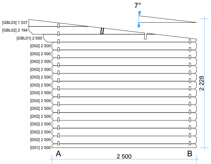
Wall D
