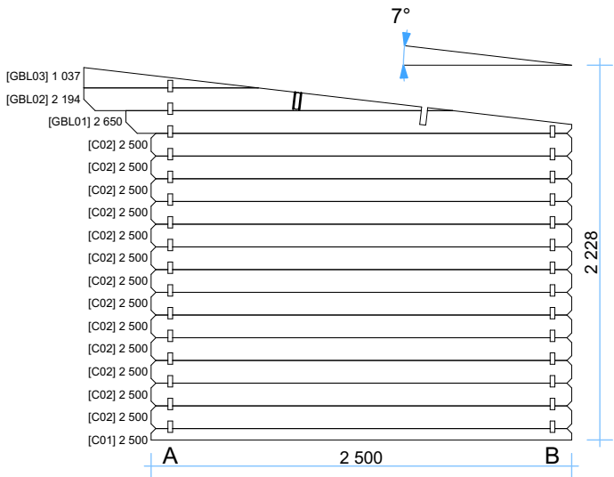
Wall C
