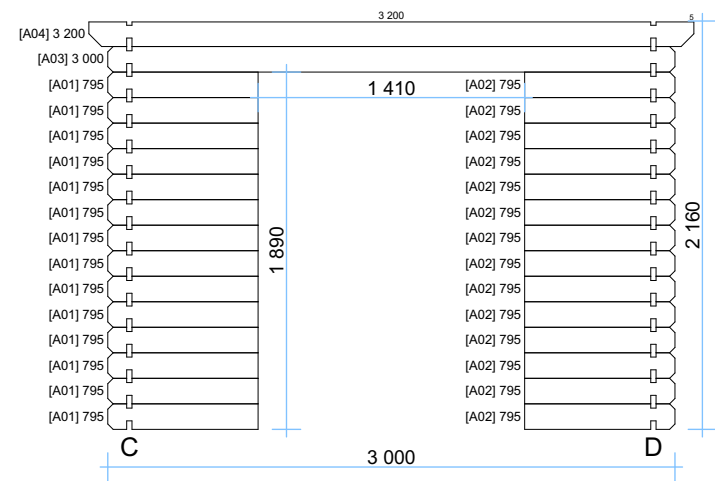
Wall B
