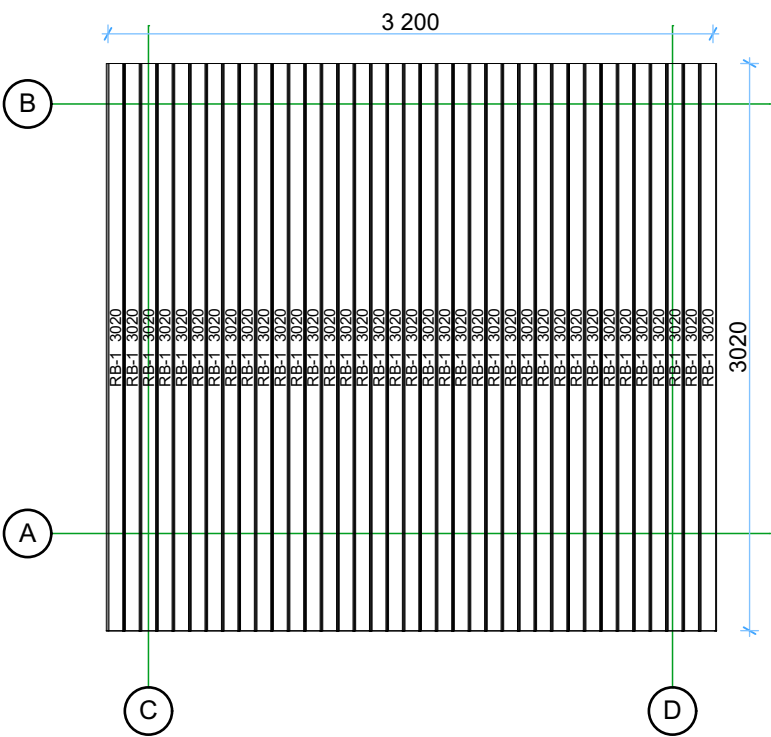
Roof boards
