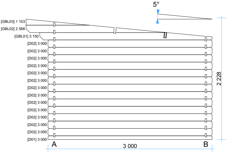
Wall D
