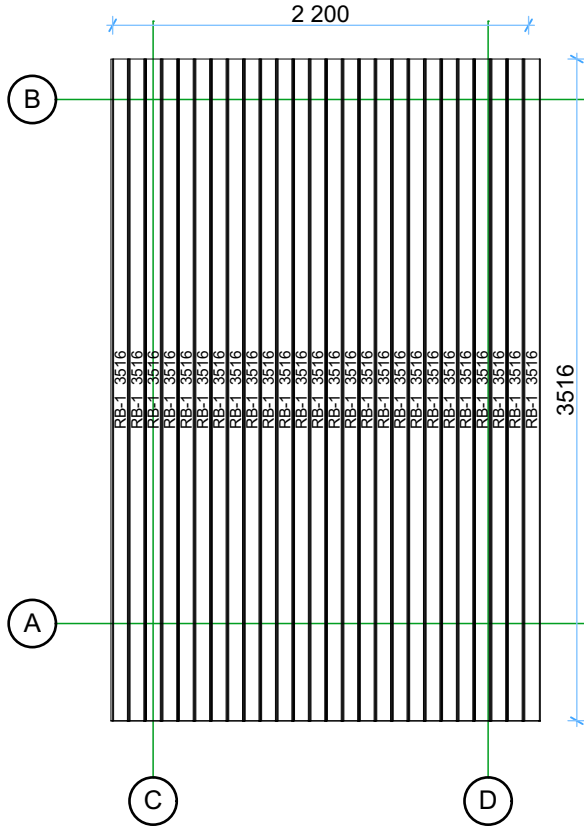
Roof boards
