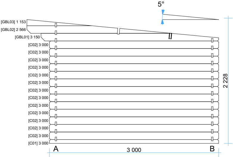
Wall C
