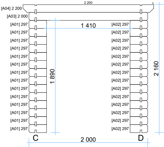
Wall B
