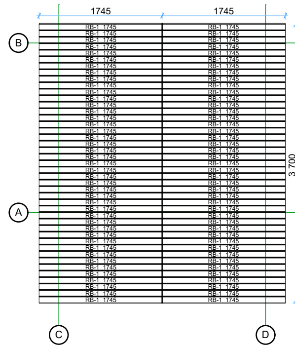
Roof boards
