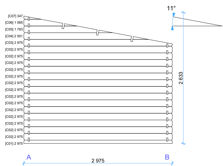
Wall D
