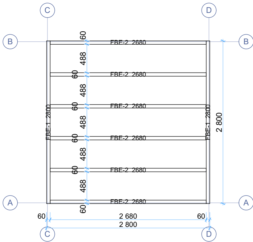
Floor bearers
