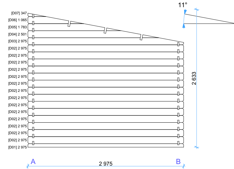
Wall D
