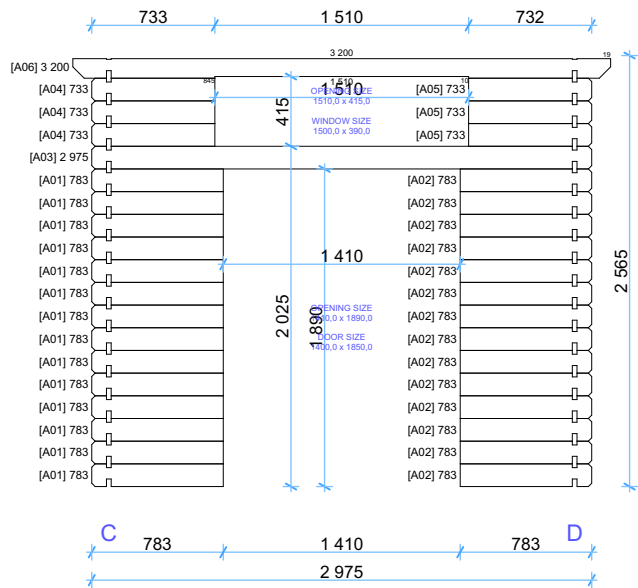
Wall B
