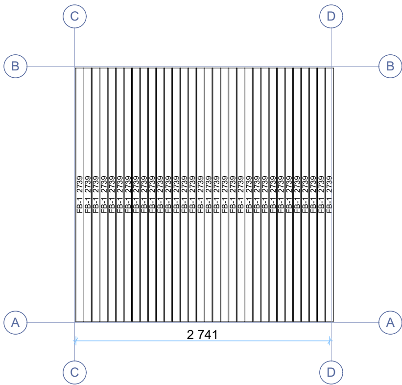
Floor boards
