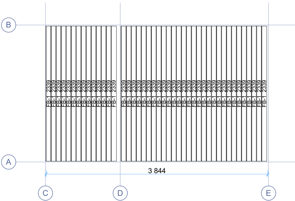
Floor boards
