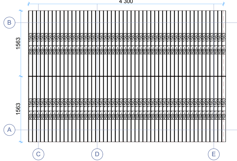
Roof boards
