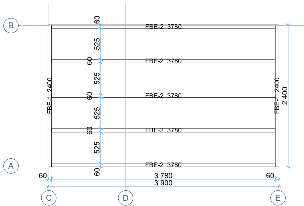
Floor bearers
