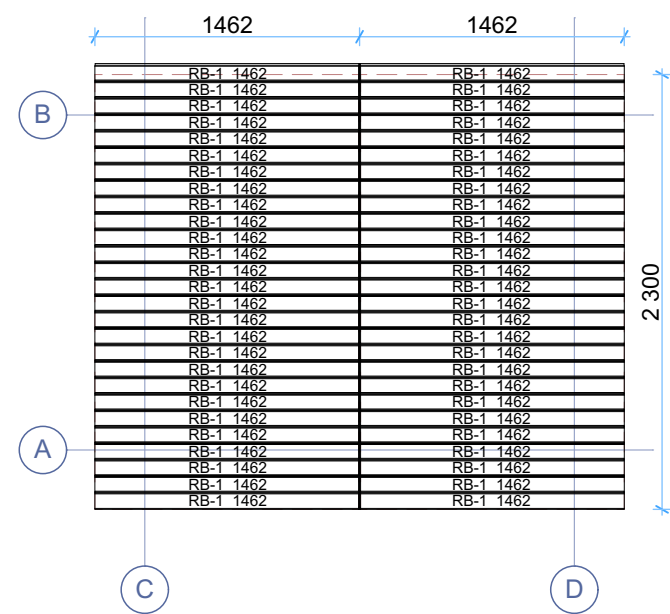
Roof boards 1:40
