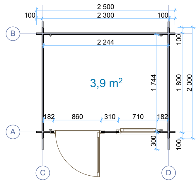
Ground floor plan 1:40
