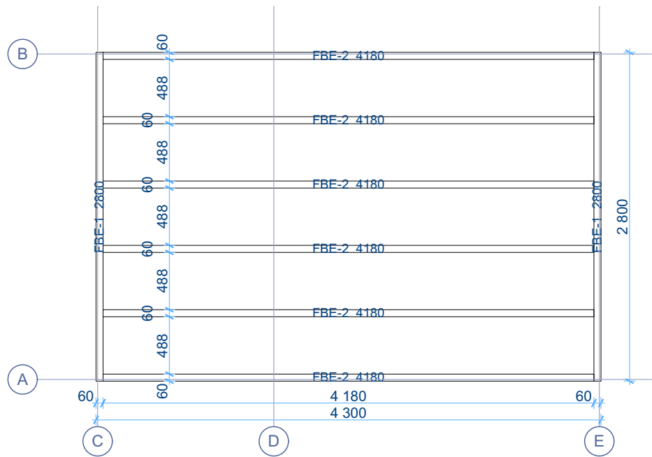
Floor bearers1:45
