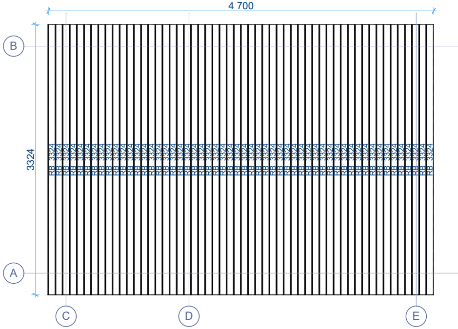
Roof boards
