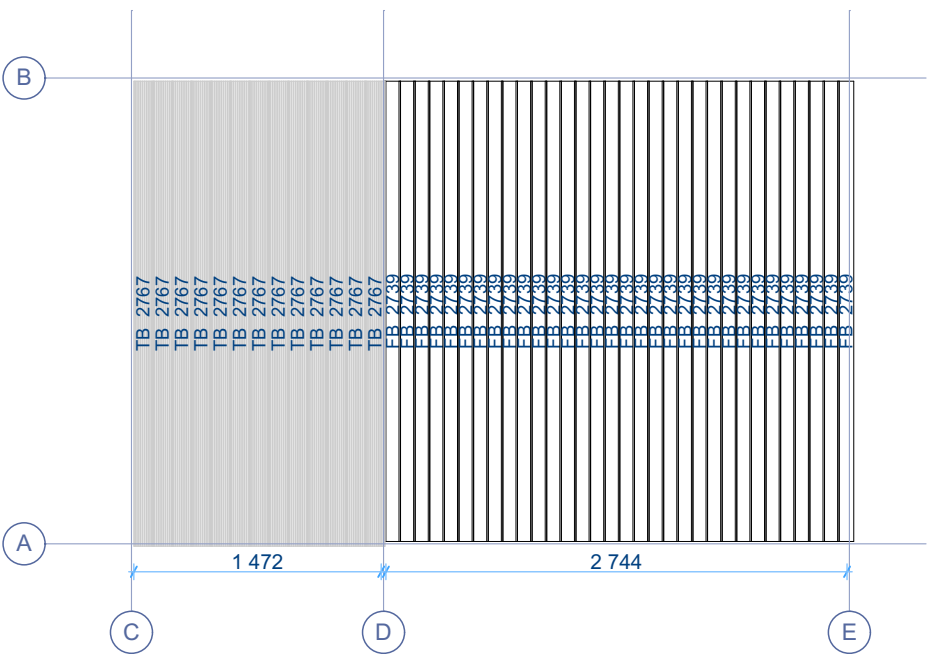
Floor boards1:45
