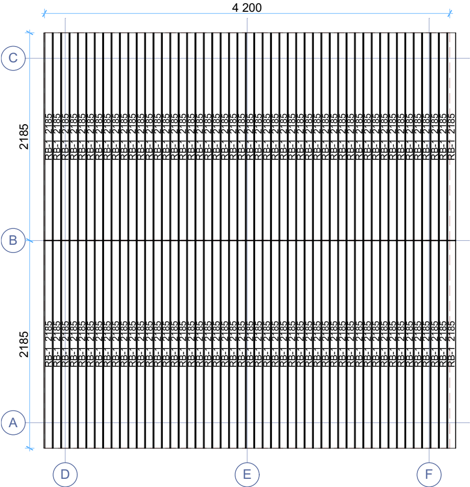
Roof boards
