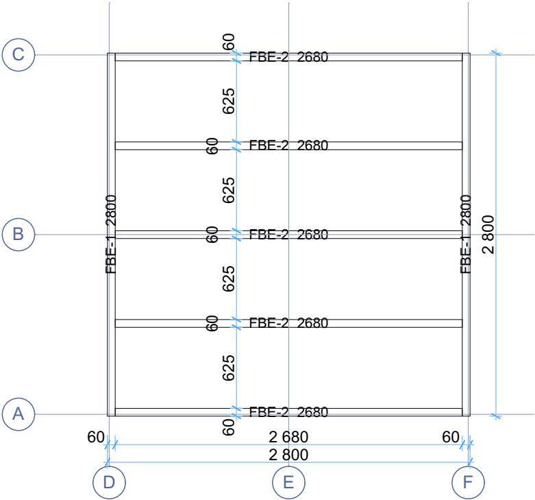
Floor bearers
