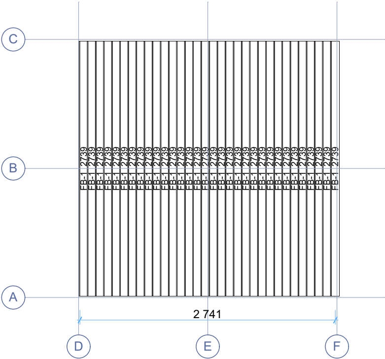
Floor boards
