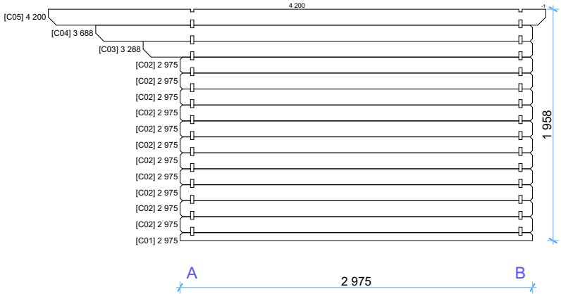
1:45 Wall D
