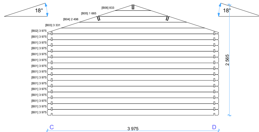
Wall B
