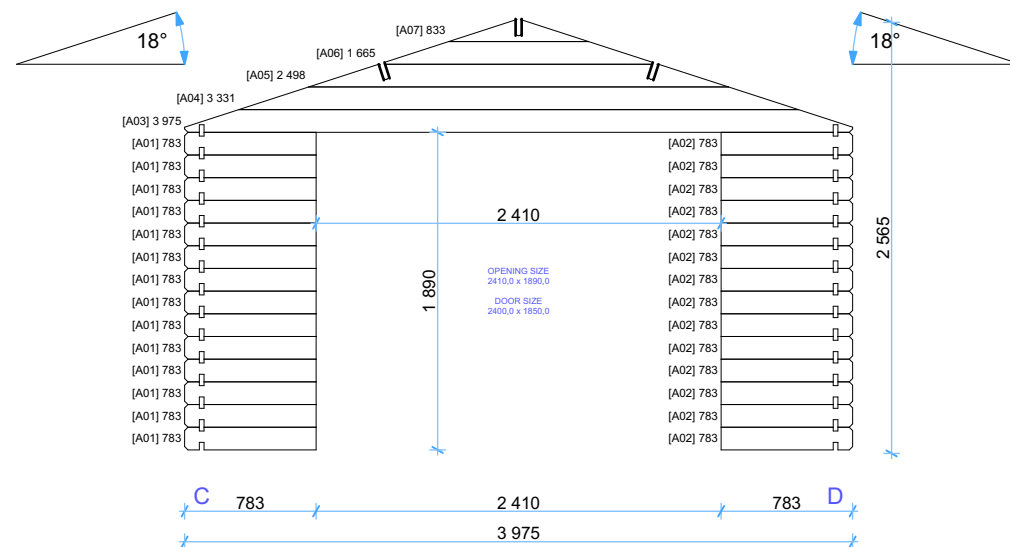
Wall B
