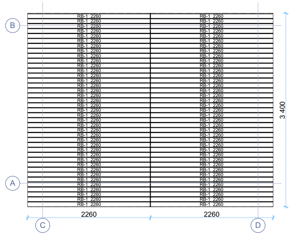
Roof boards
