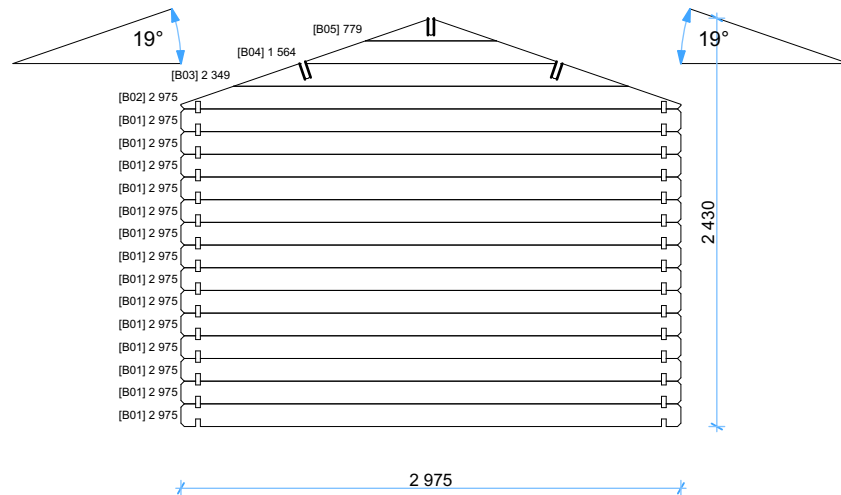
Wall B
