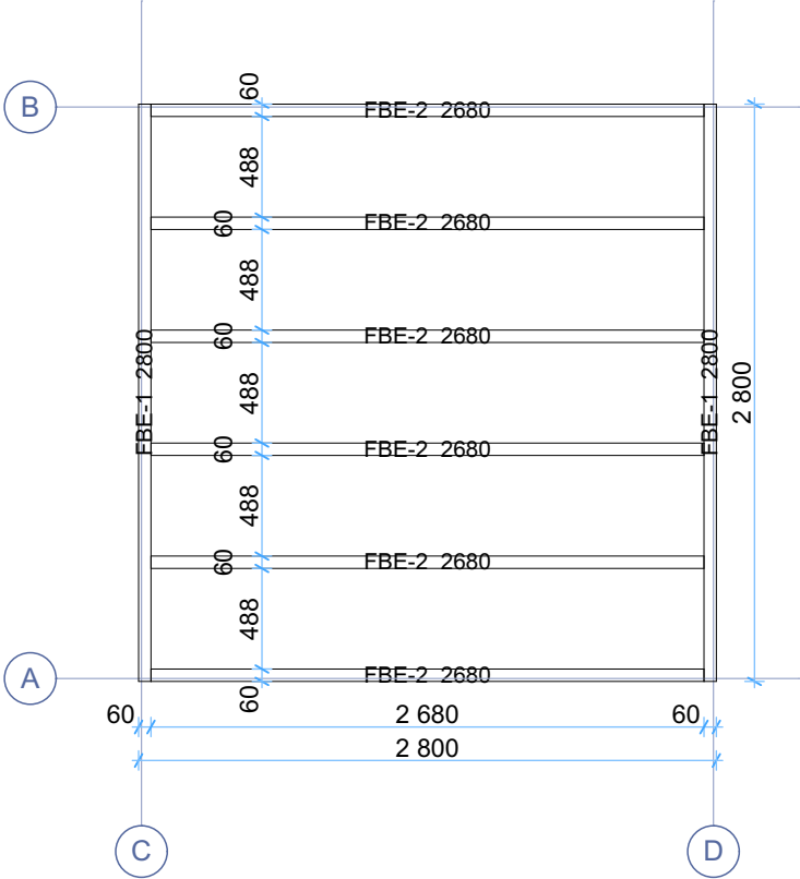
Floor bearers 1:40
