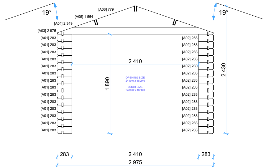
Wall A
