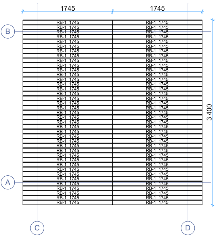
Roof boards
