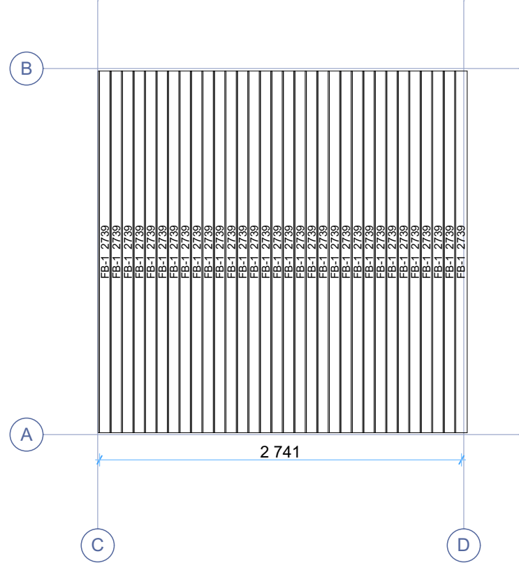
Floor boards 1:40
