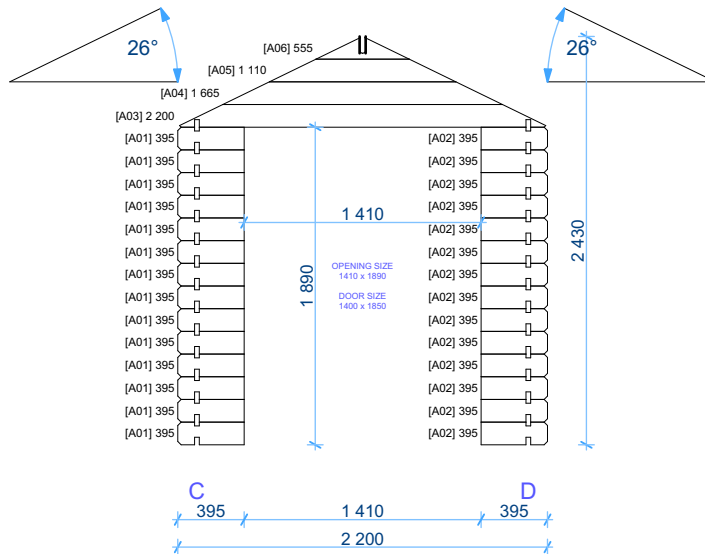
Wall A
