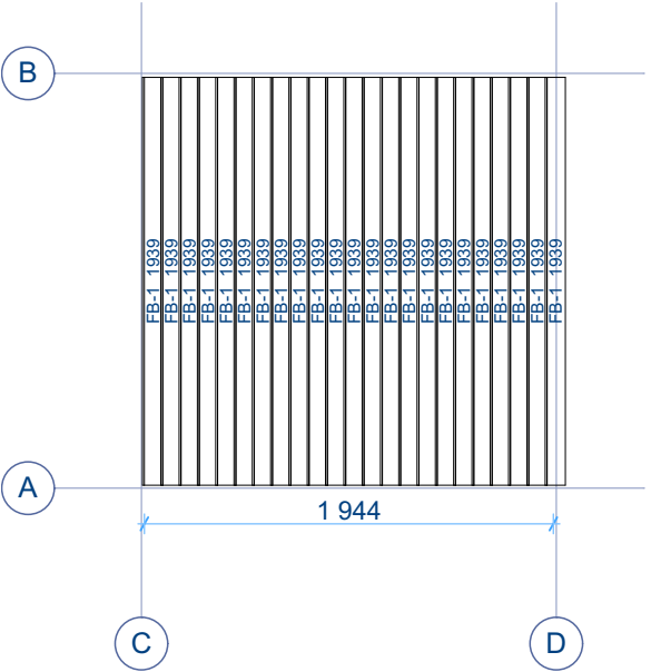
Floor boards
