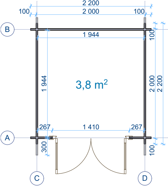
Ground floor plan 1:40
