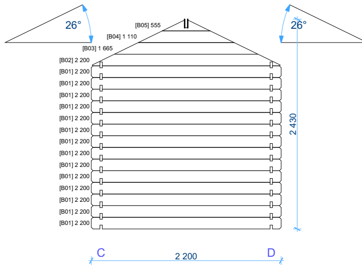
Wall B
