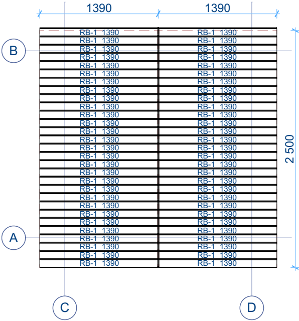
Roof boards 1:40
