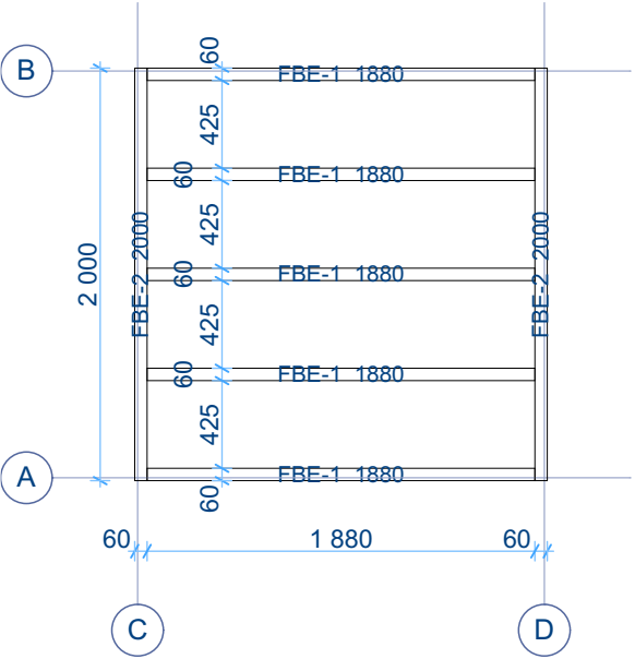
Floor bearers
