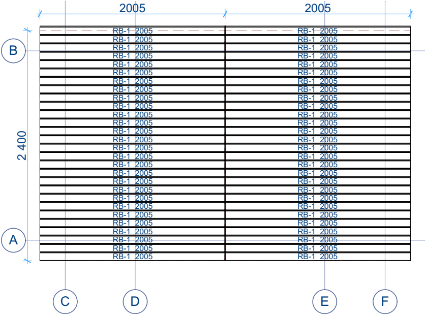
Roof boards
