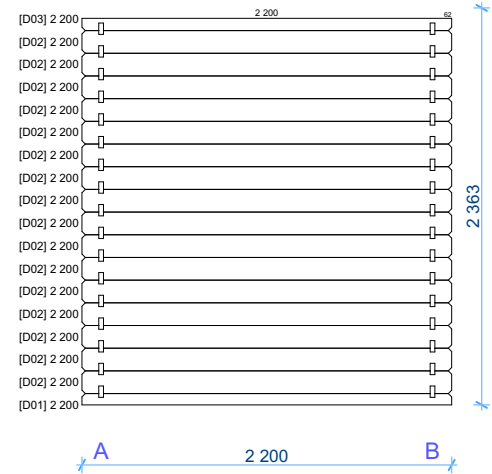
Wall D 1:45
