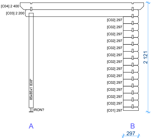
Wall D 1:45
