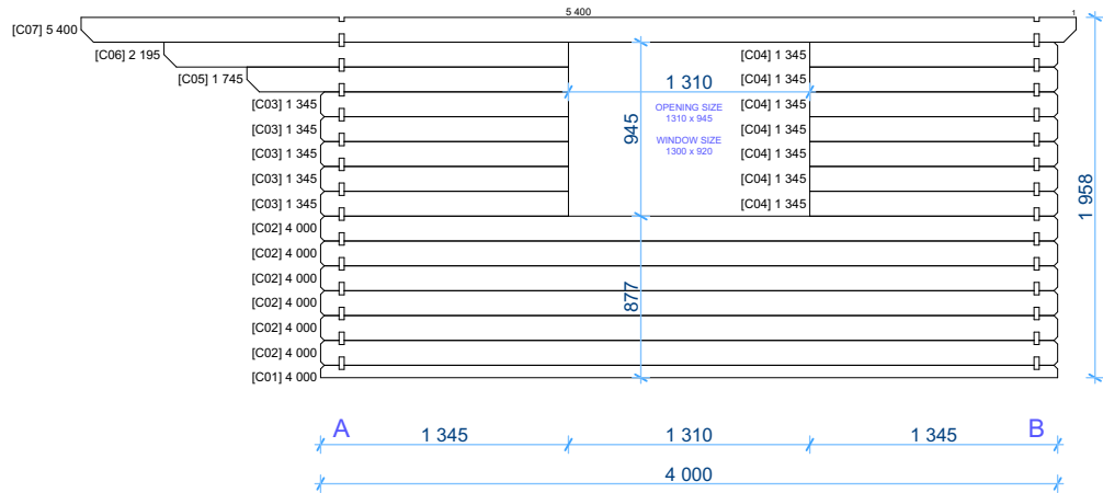
1:45 Wall D
