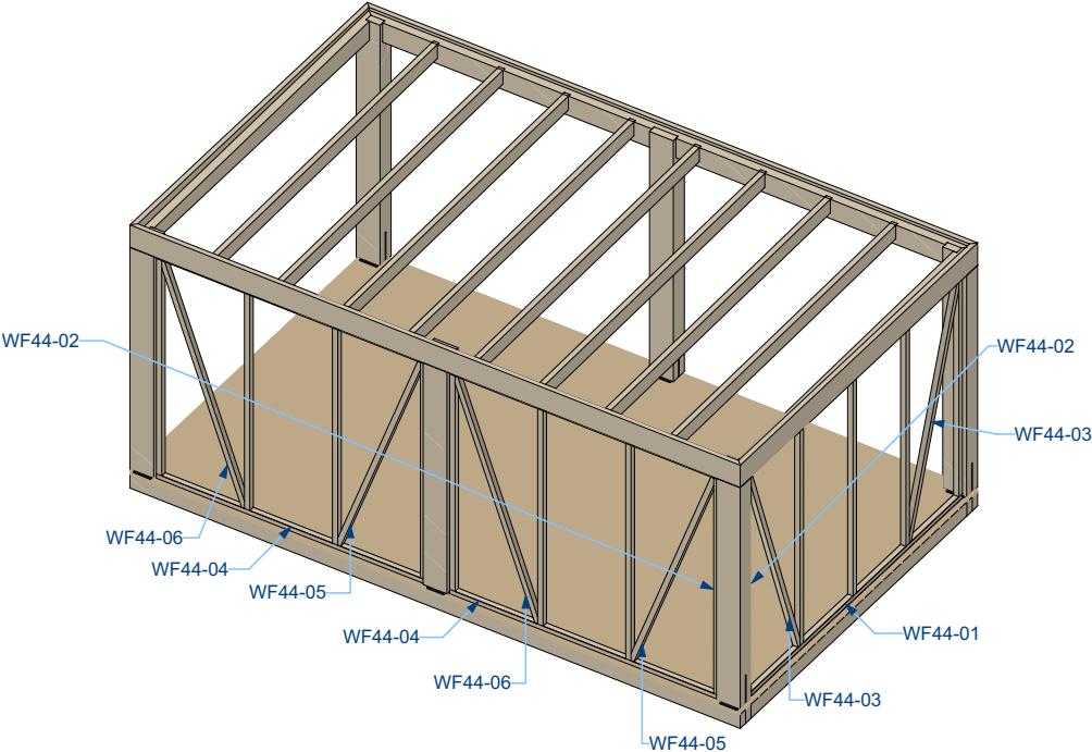
Wall frame 44x44 (2)
