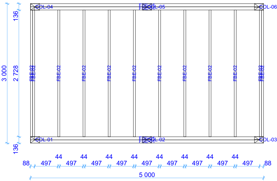
Floor bearers 1:50
