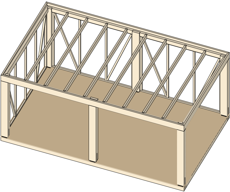
Wall frame 44x44 (1)
