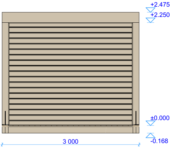
Left Elevation
