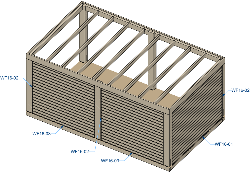
Wall frame 16x16
