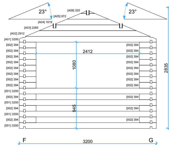
Wall D
