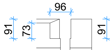
W-01-1 1:10
