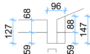
W-01-2 1:10
