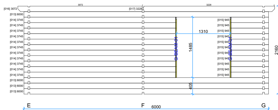
Wall D
