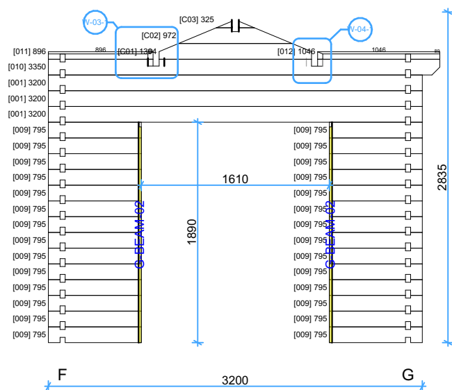
Wall C
