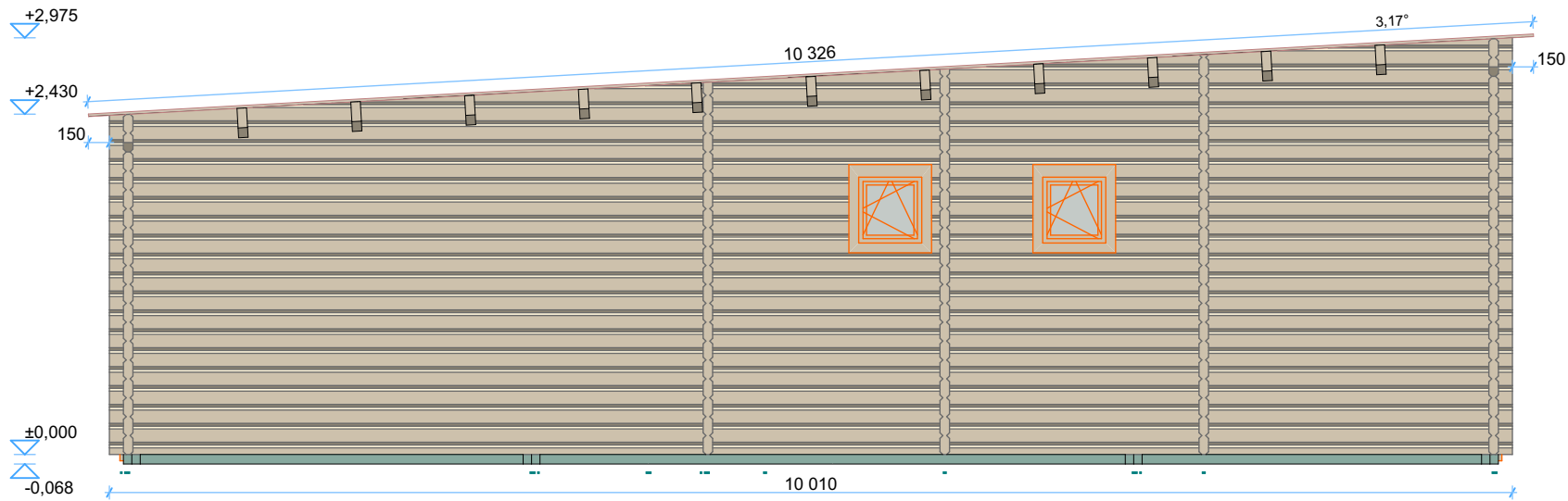
Left Elevation
