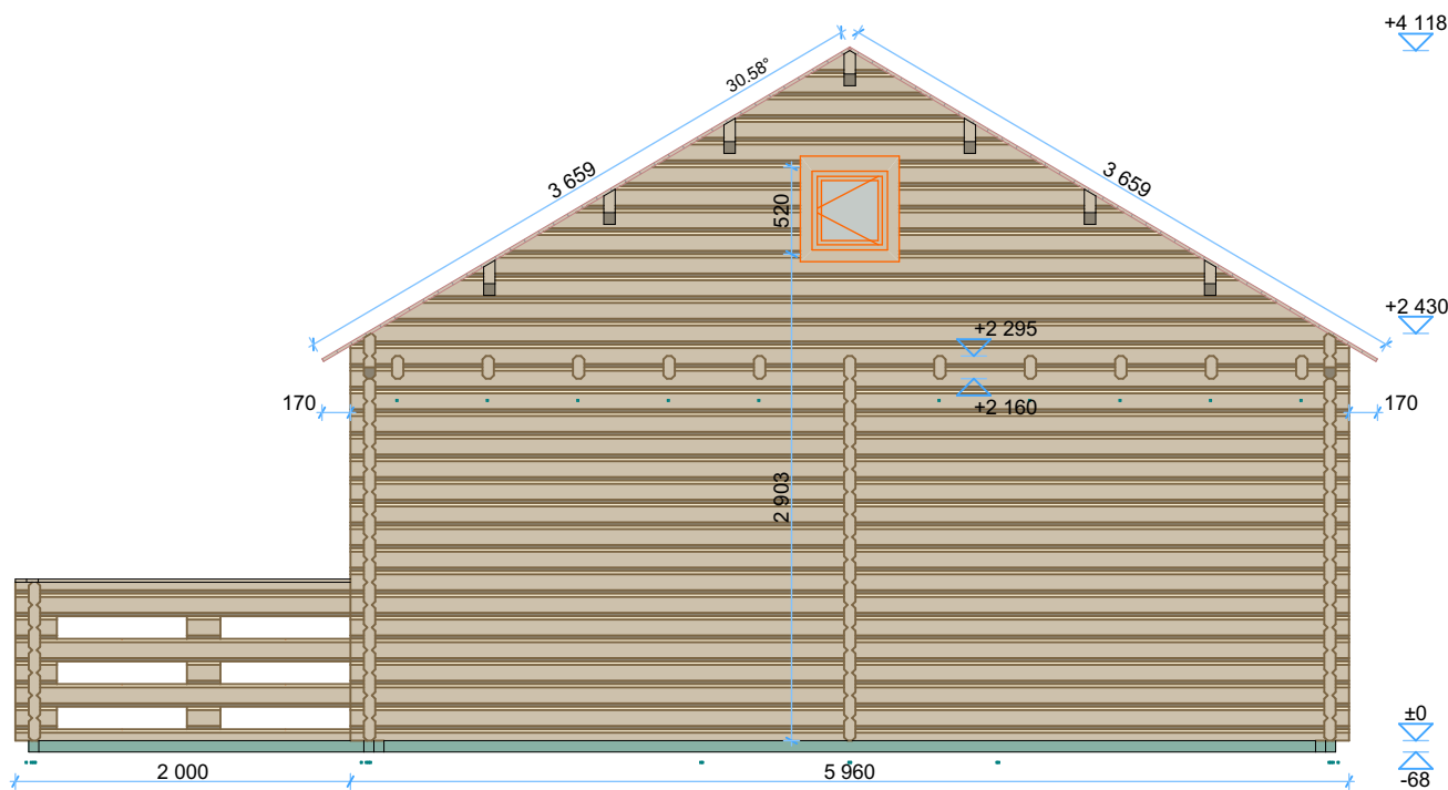
Back Elevation
