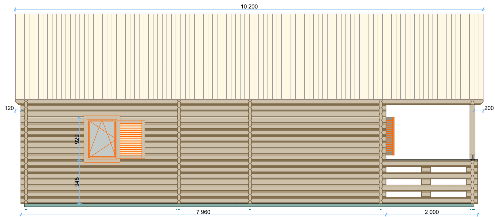
Left Elevation
