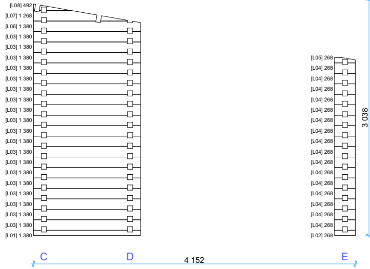
Wall L 1:50
