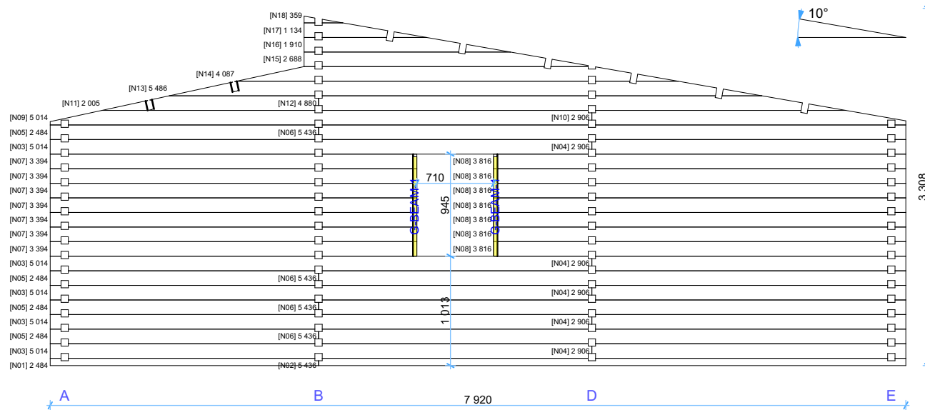
Wall N 1:50
