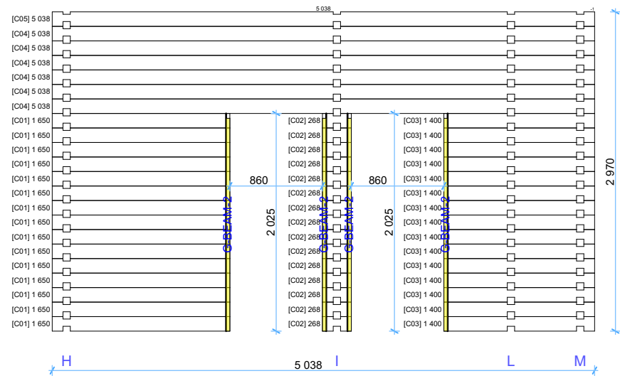
Wall C
