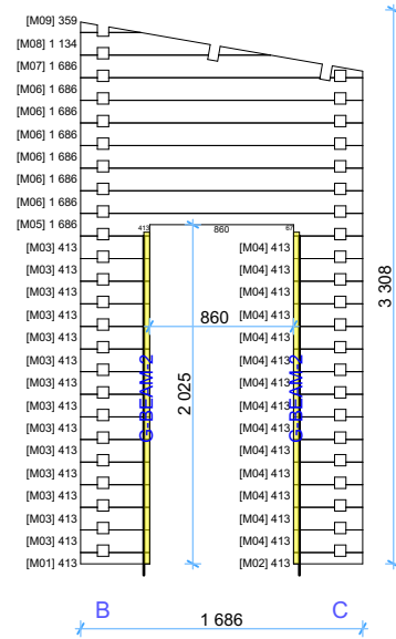
Wall N 1:50
