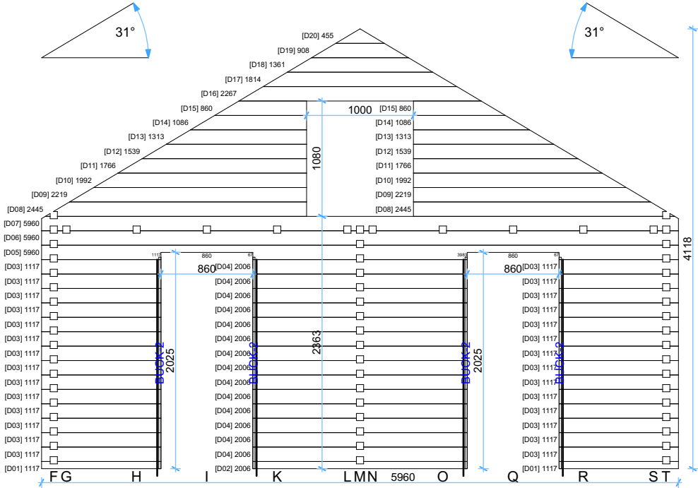
Wall D
