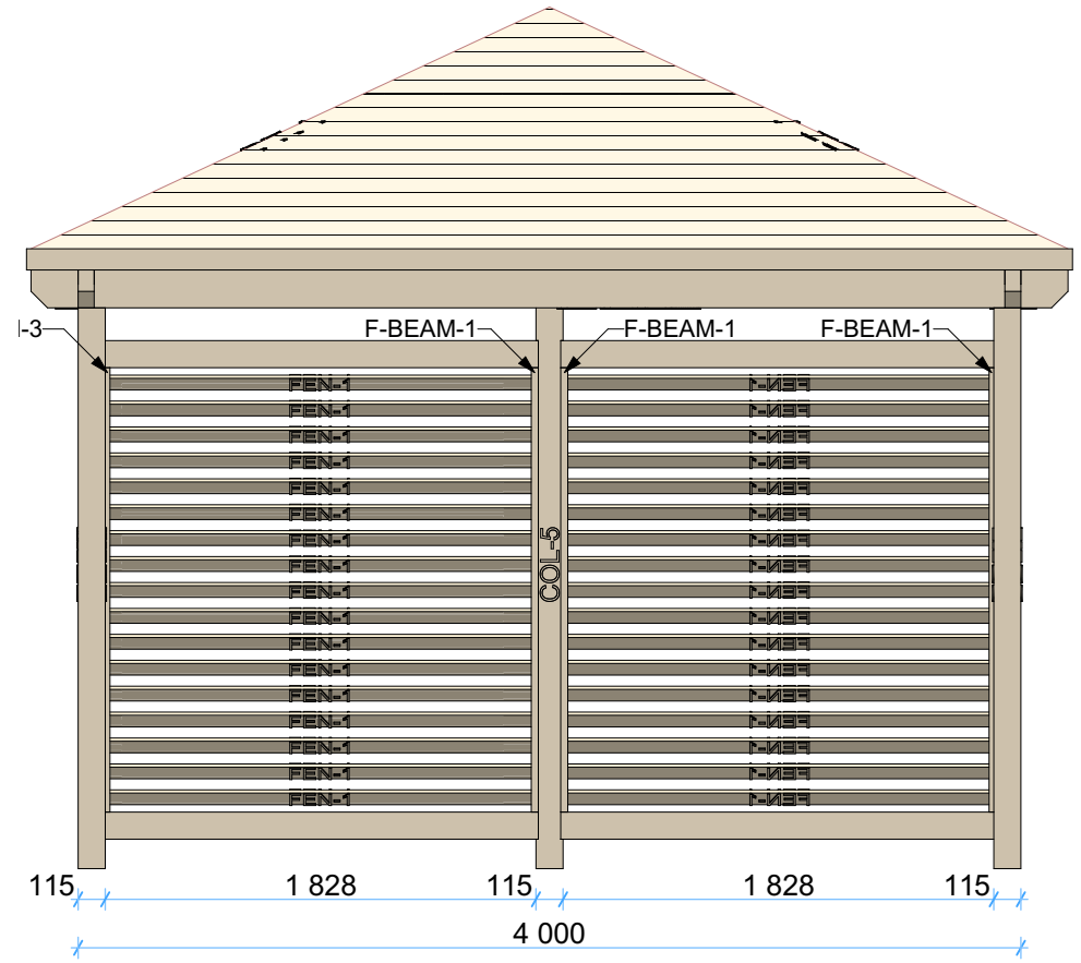
Front Elevation
