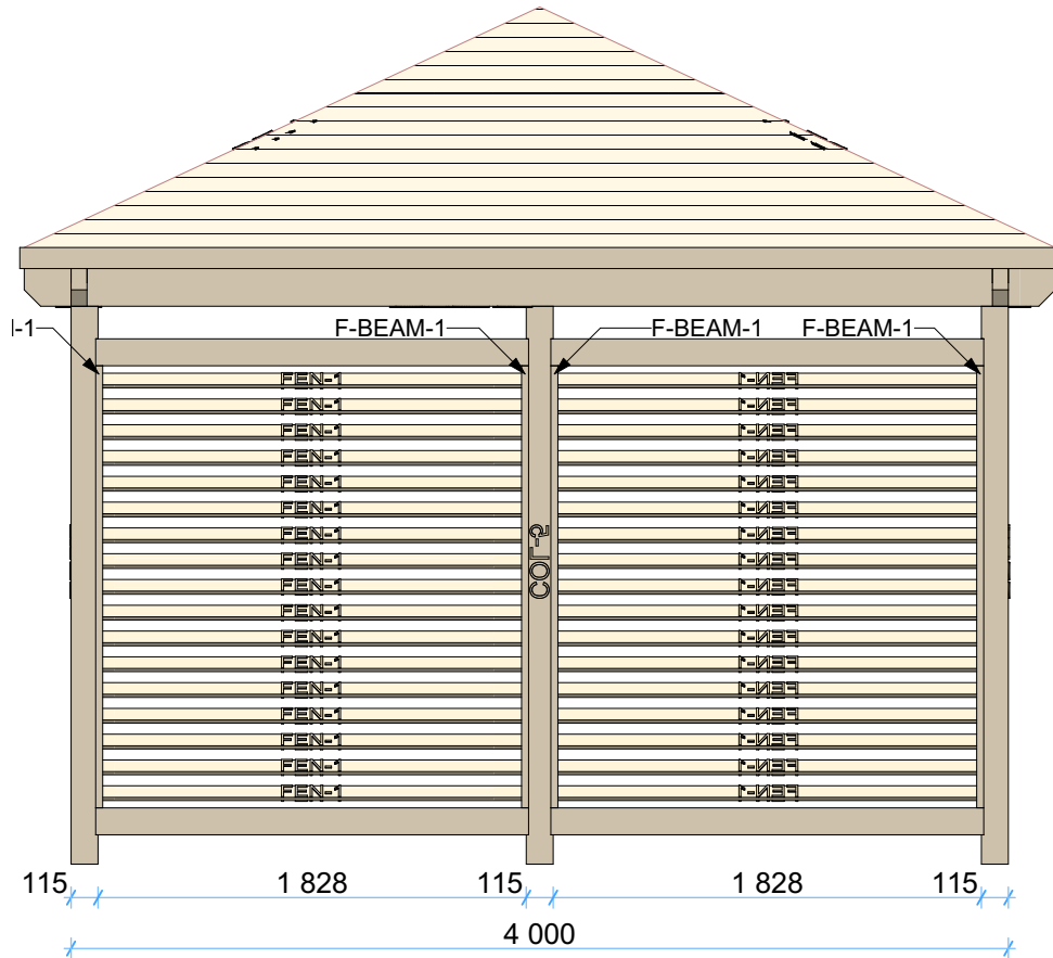
Back Elevation
