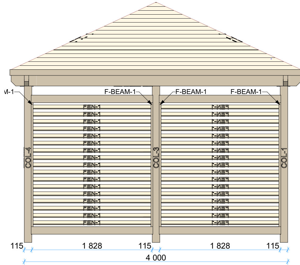
Left Elevation
