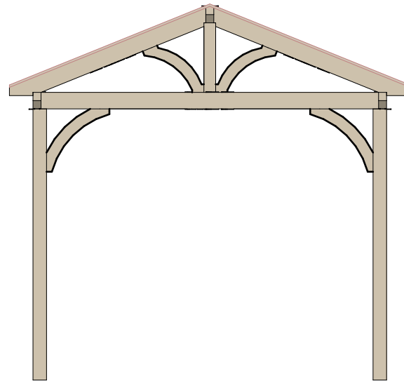
Left Elevation
