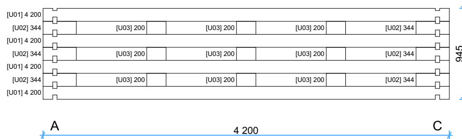
Wall U 1:40
