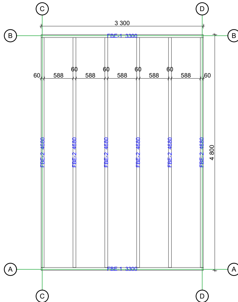
Floor bearers
