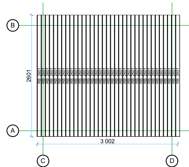
Roof boards 1:50
