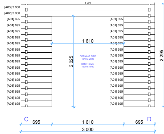
Wall B
