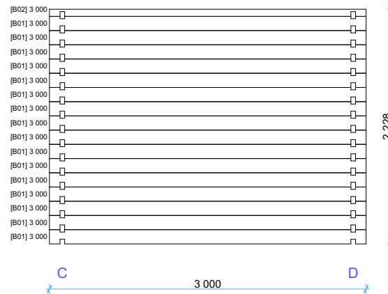
Wall B
