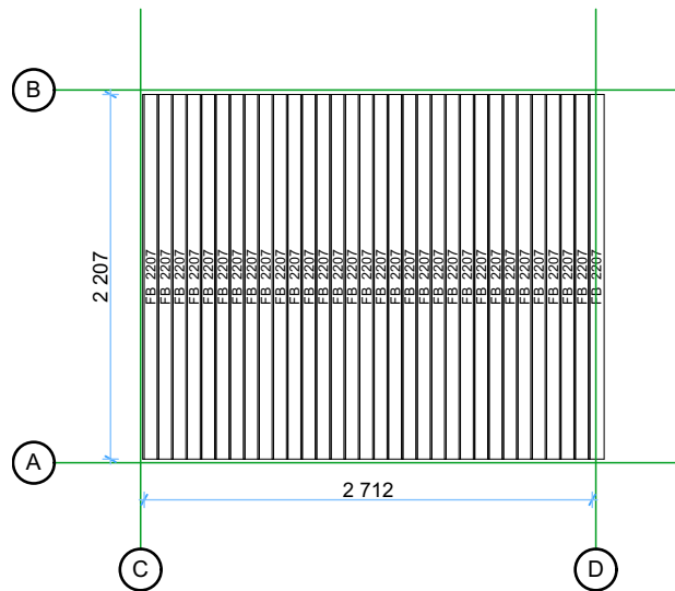
Floor boards 1:50
