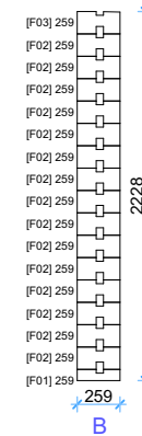
Wall F 1:50
