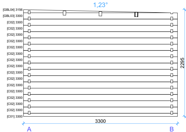
Wall C
