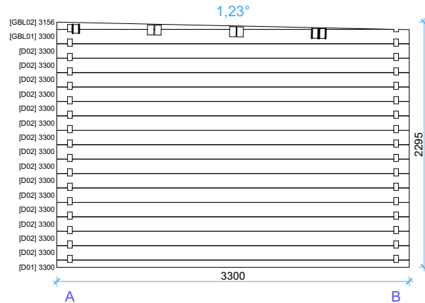
Wall D
