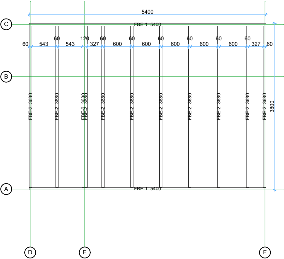
Floor bearers
