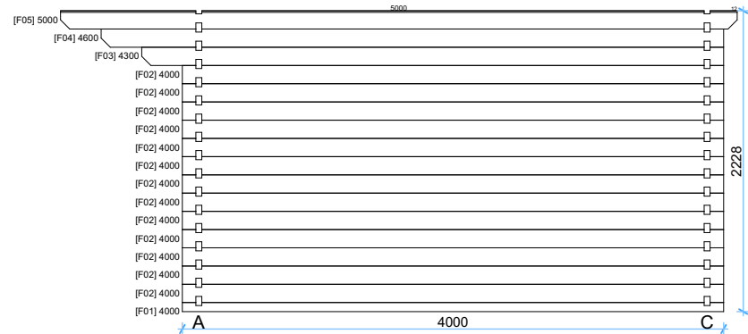
Wall F
