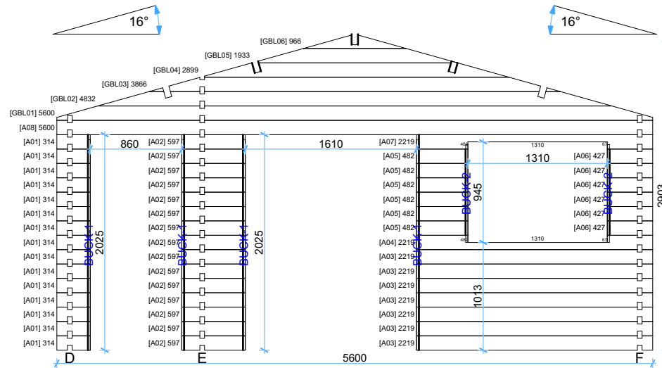
Wall C
