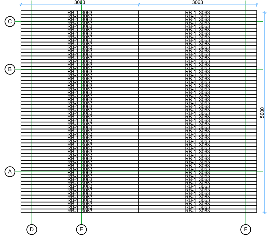
Roof boards
