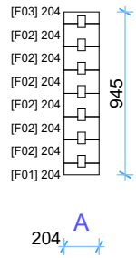
Wall H 1:40
