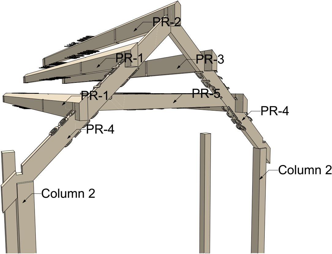
Purlins Detailed
