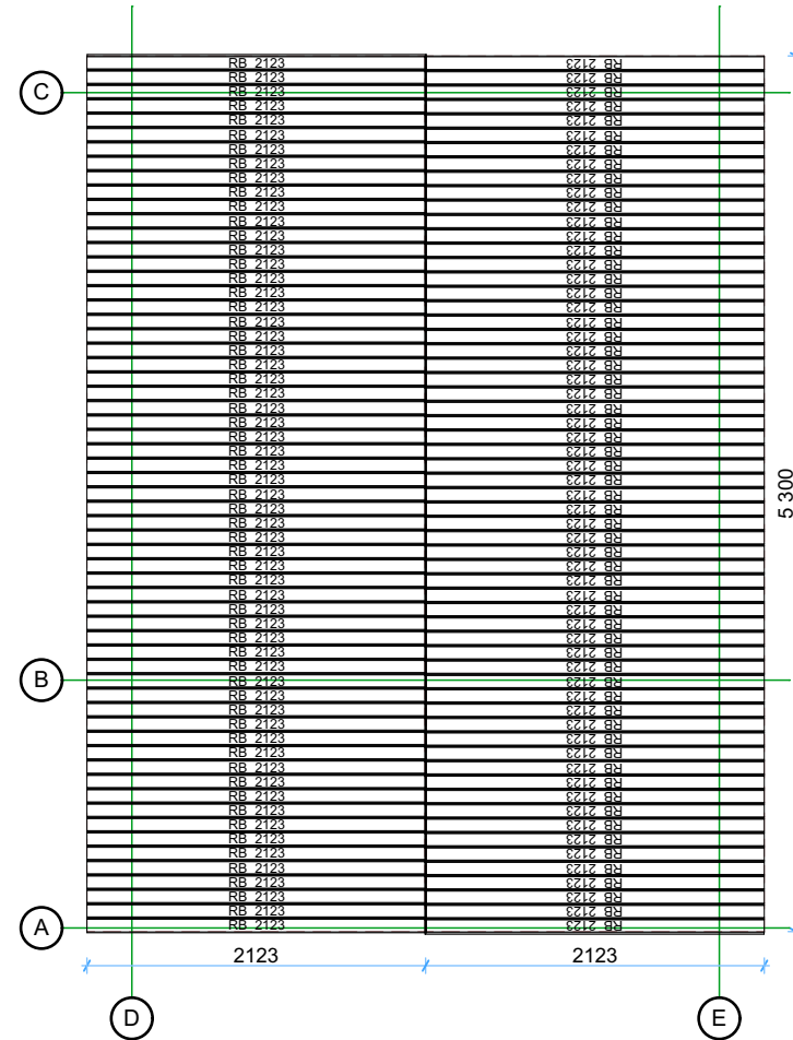
Roof boards
