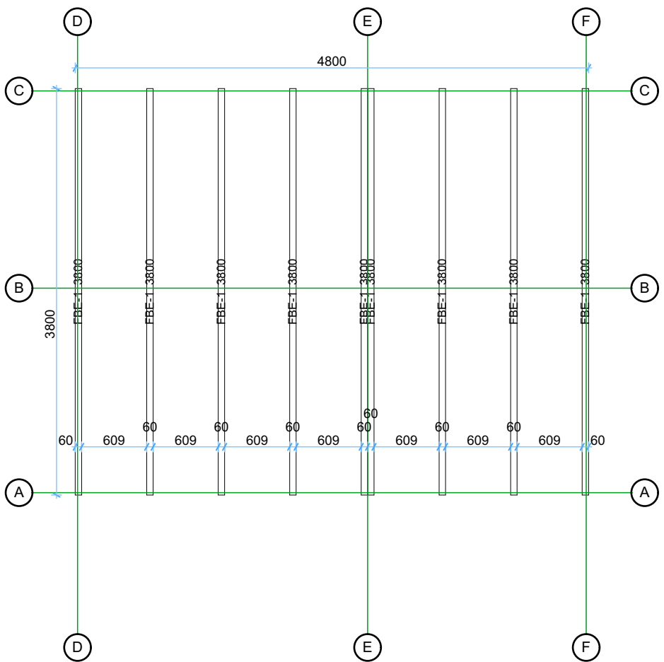
Floor bearers 1:50
