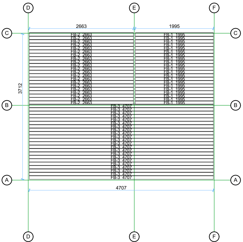
Floor boards 1:50
