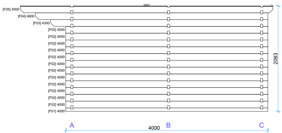
Wall F
