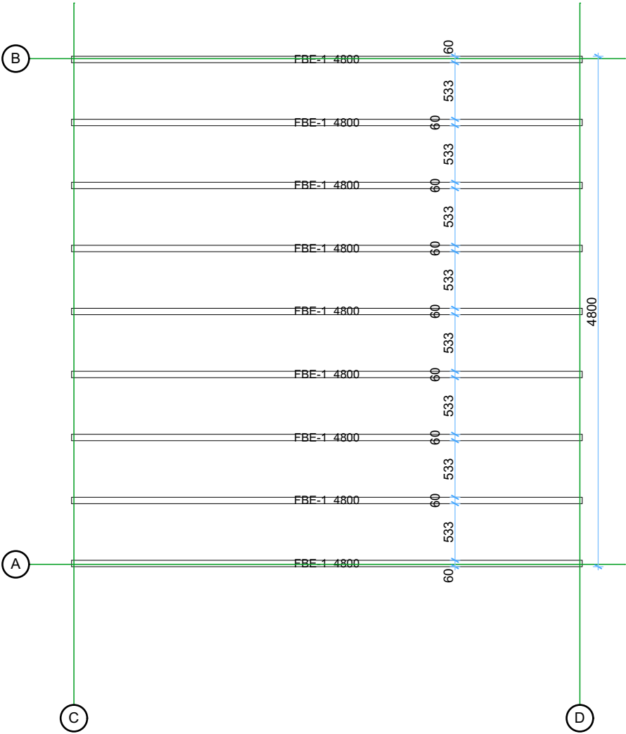
Floor bearers
