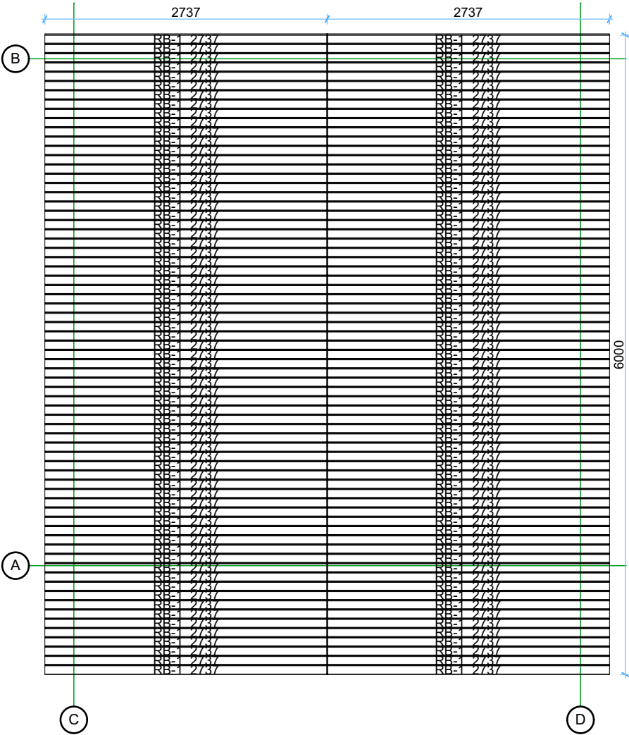
Roof boards
